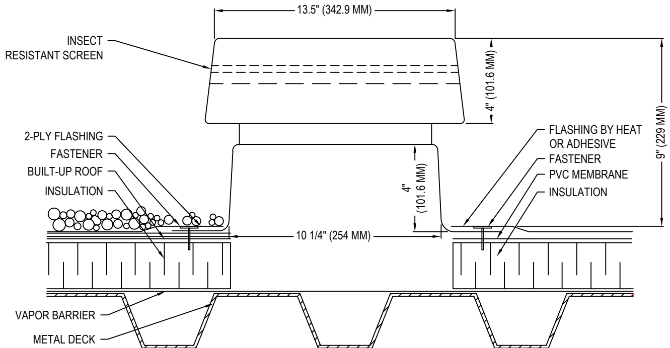
SECTION
