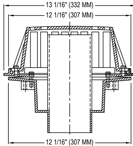
SIDE SECTION
