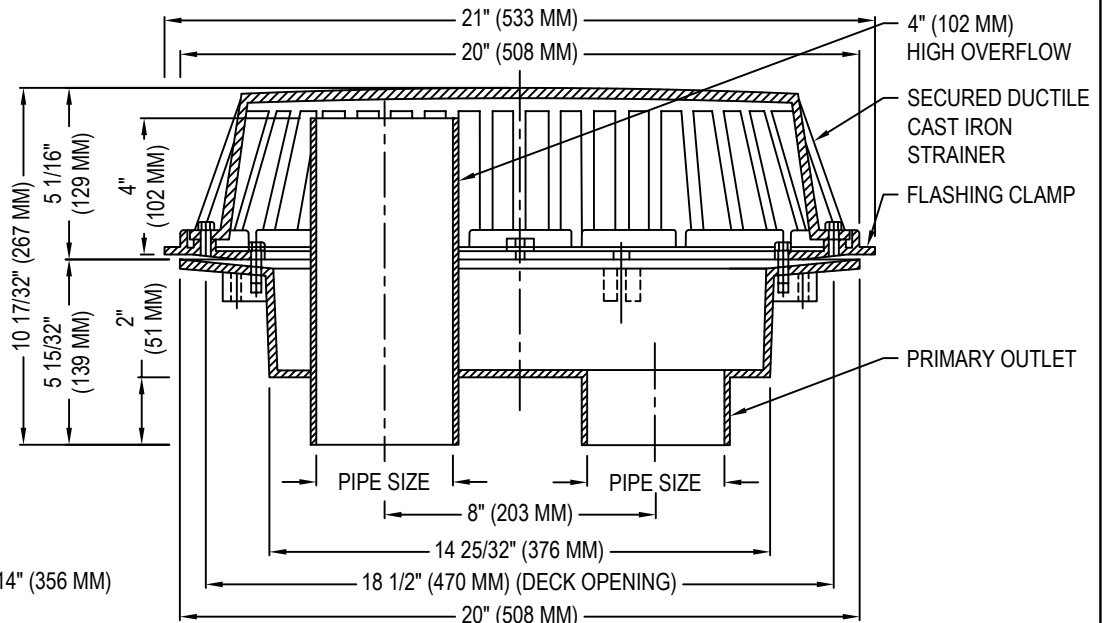
FRONT SECTION
