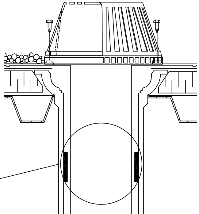
SECTION COMPRESSED SEAL
